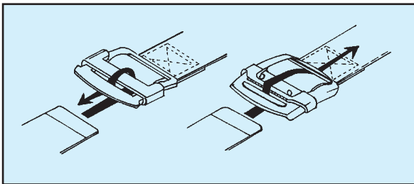
FOLDING-BACK BUCKLE
